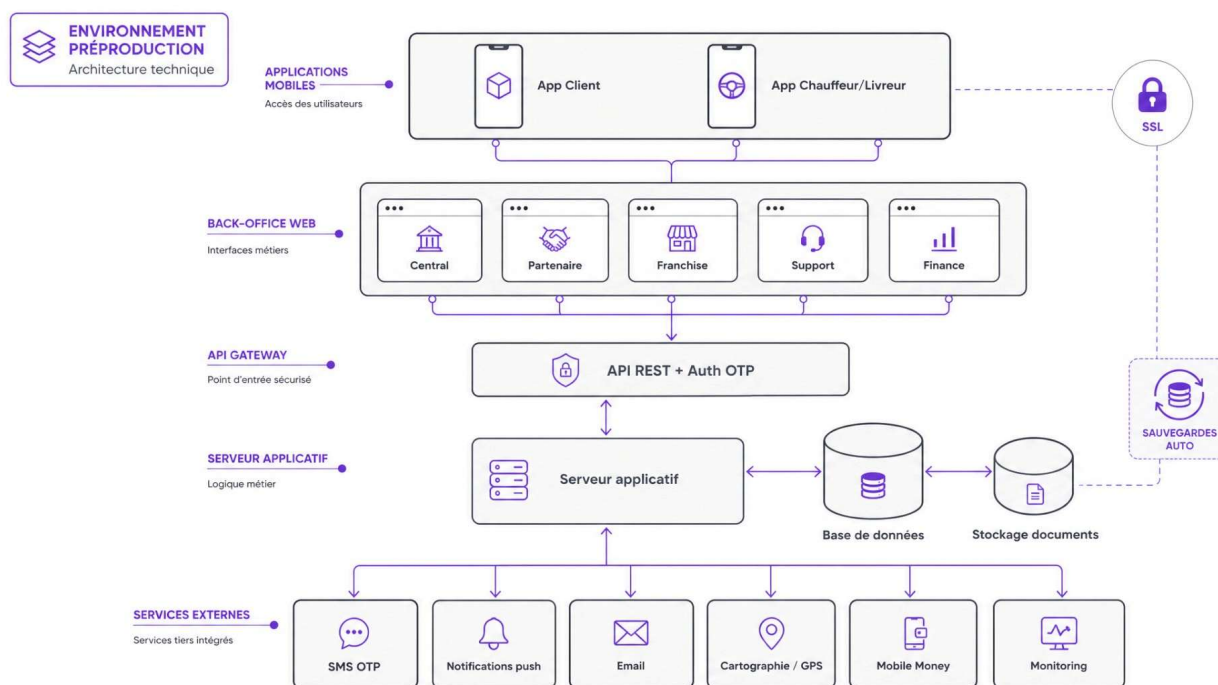
Fig. 22.1 — Schéma d'architecture préproduction (applications mobiles, back-office web, API, BDD, stockage, services externes)
